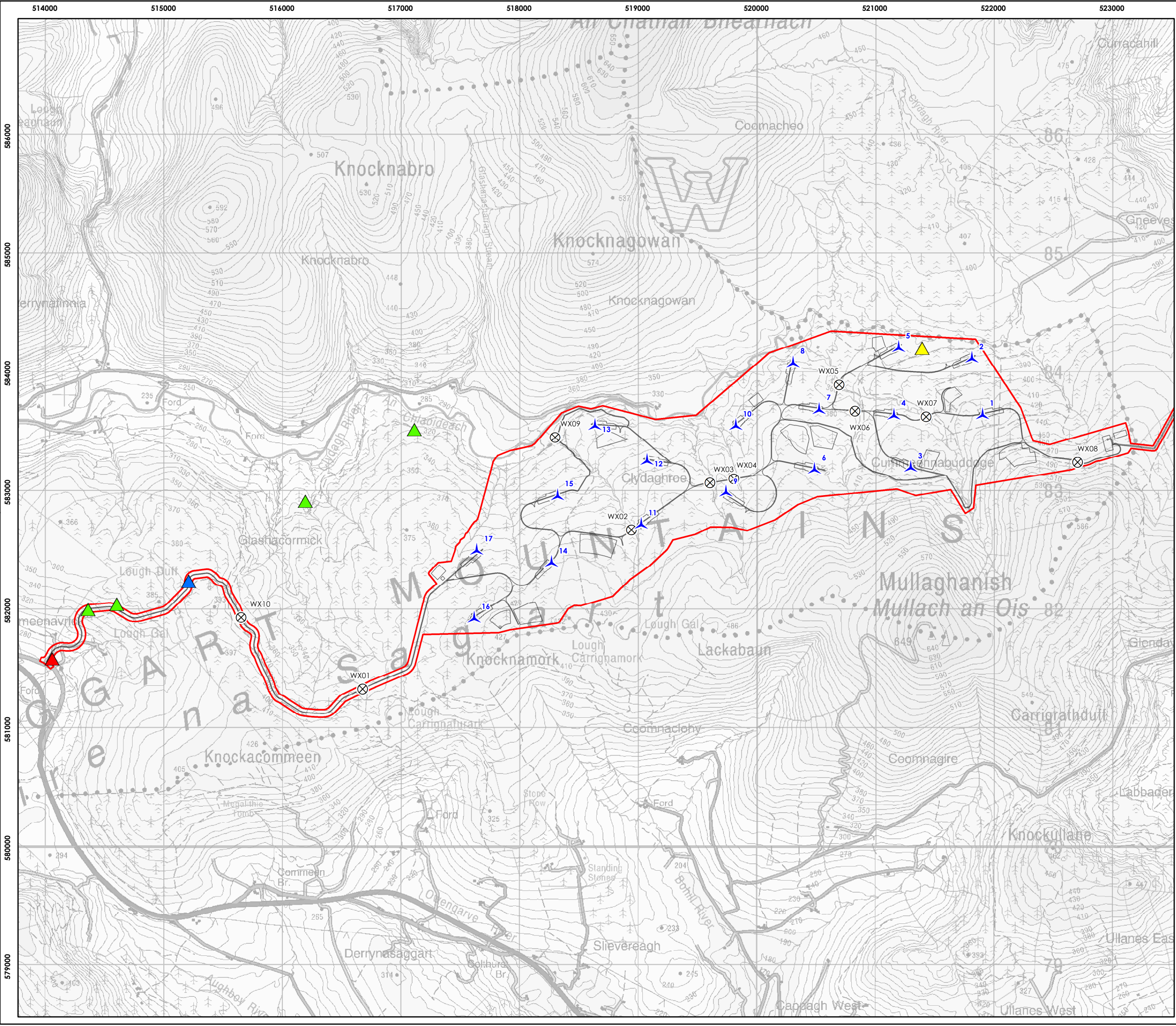
Figure 8-3 Invasive Species
